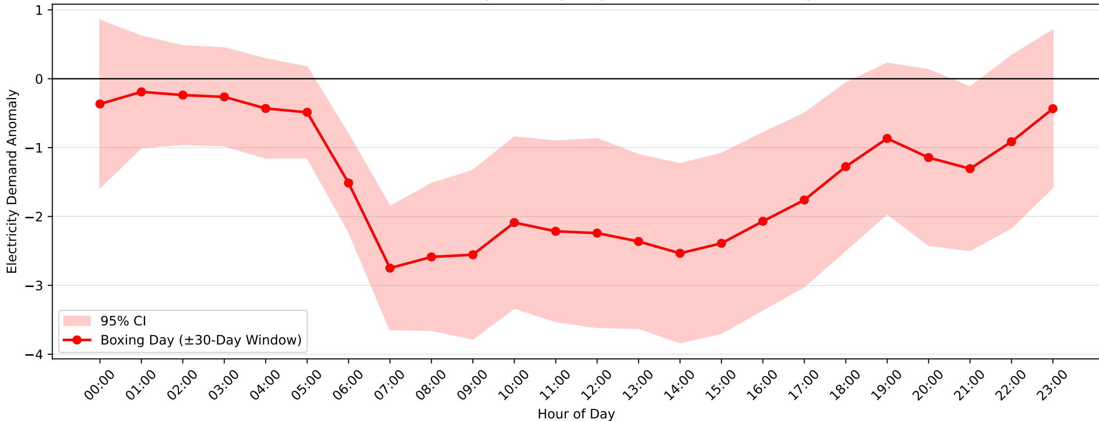
Arncliffe Demand Anomaly: Boxing Day (2004–2017, \pm 30 -Day Window)
